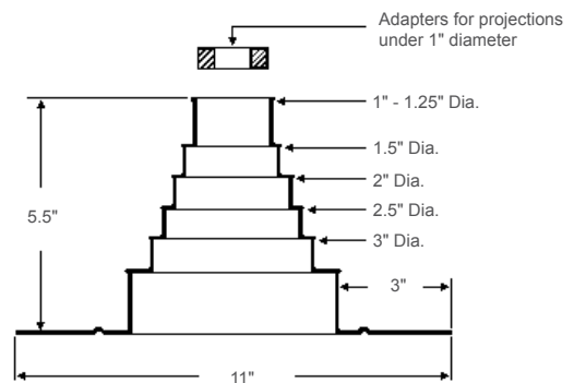
Small Retrofit
