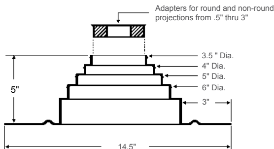
Large Retrofit
