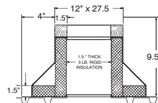
RC-4A For Decks with Rigid Insulation
