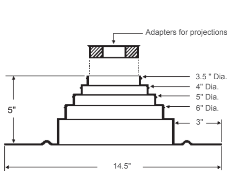
Large Retrofit
