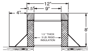
RC-3A For Noninsulated Decks
