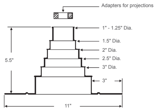
Small Retrofit
